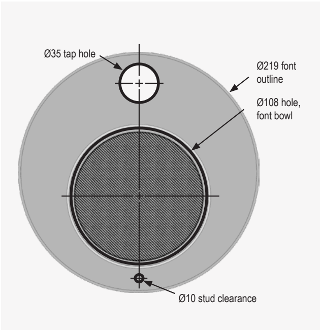
INTEGRATED FONT FOR CLASSIC AND ELITE
