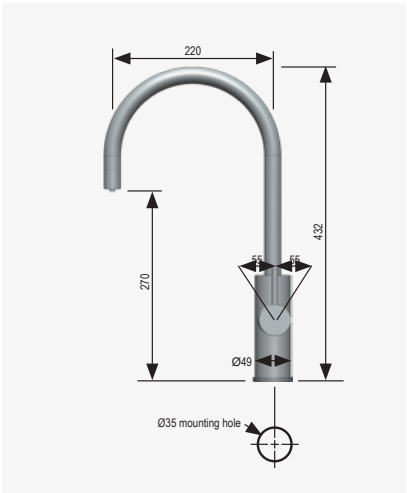
ARC MIXER
