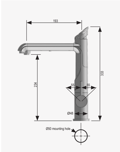
ALL-IN-ONE CLASSIC
