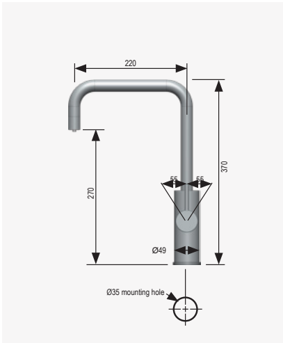
CUBE MIXER
